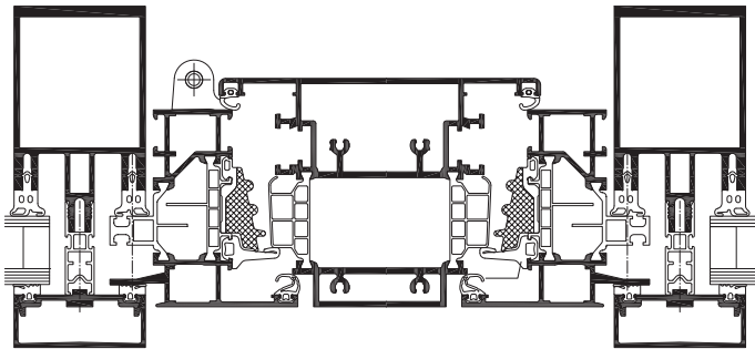
WICLINE 75 evo ventilation flap 250
